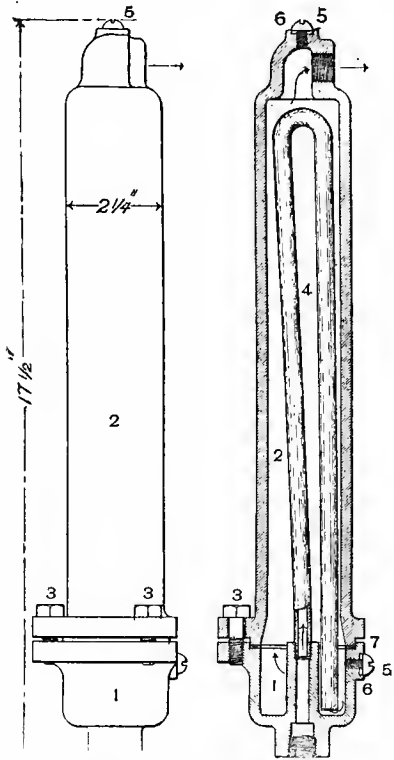
Figs. 3119-3120. Elevation and Section. MERCURIAL CHECK-VALVE.
